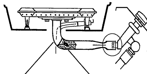
VENTURI TUBE
